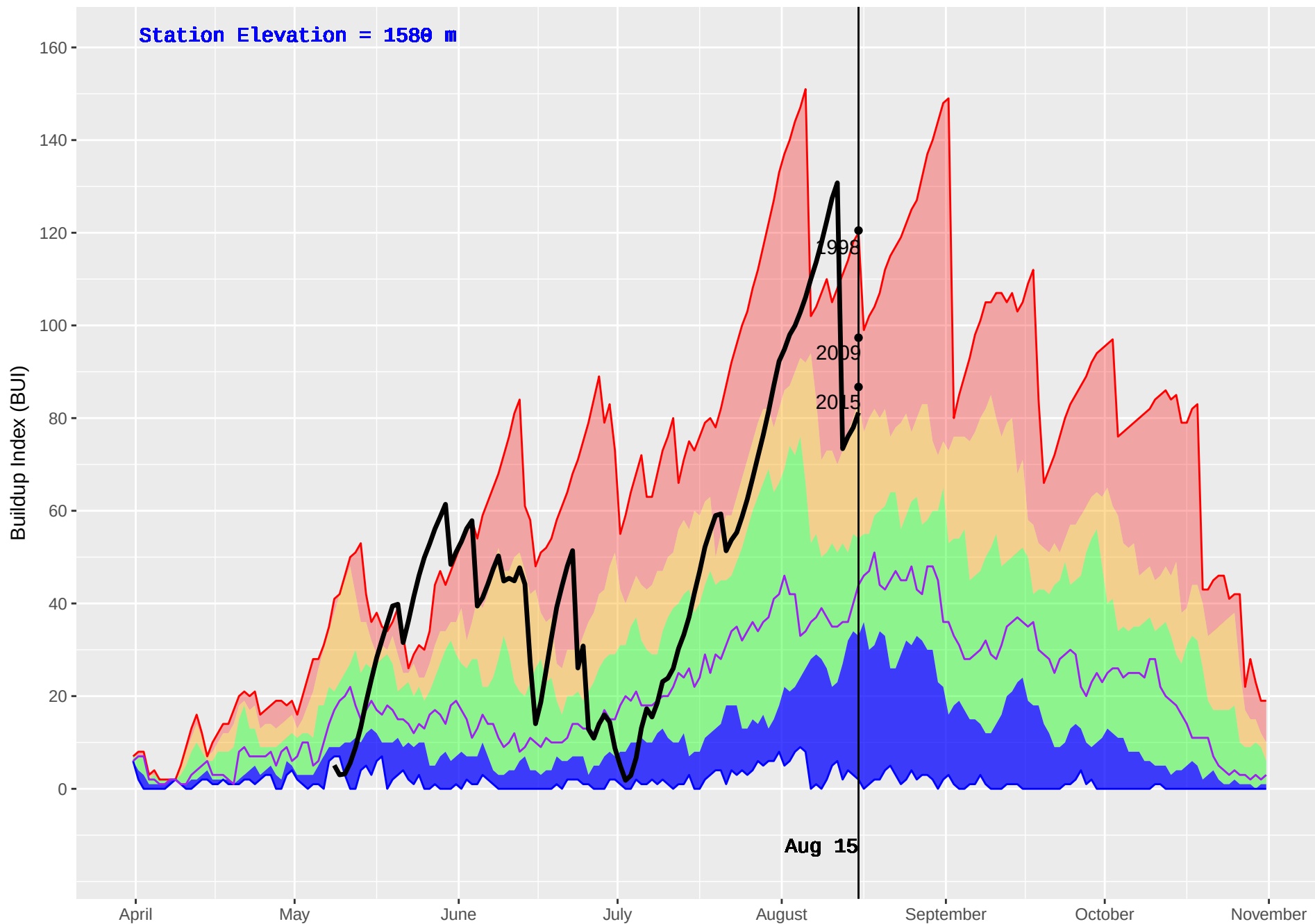
WINDY MOUNTAIN (244) : Historical (1989–2016) and Current (2018) Daily Buildup Index (BUI)
